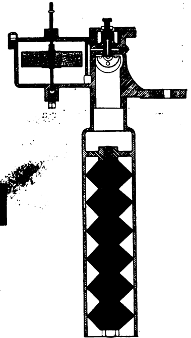
VERTICAL SECTION OF CARBURETER.
